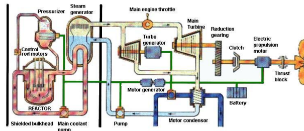
Pressurized-water Naval Nuclear Propulsion System
